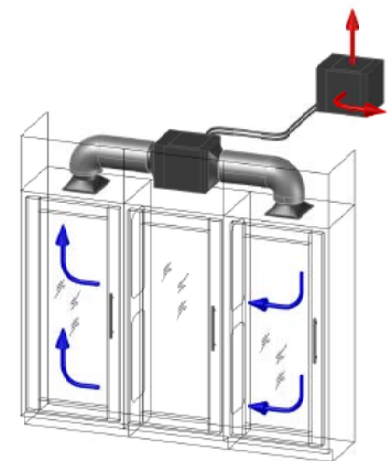
DUCTED-SPLIT
